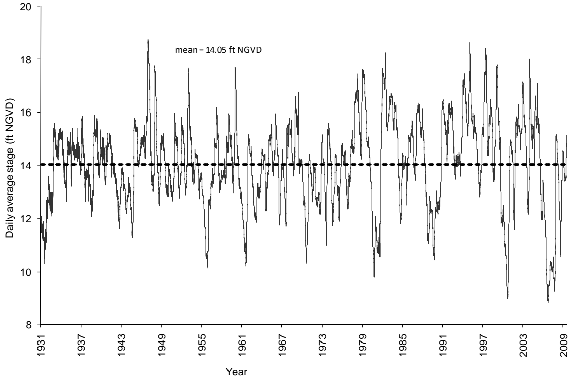
Figure 9. Daily average stage for Lake Okeechobee.
