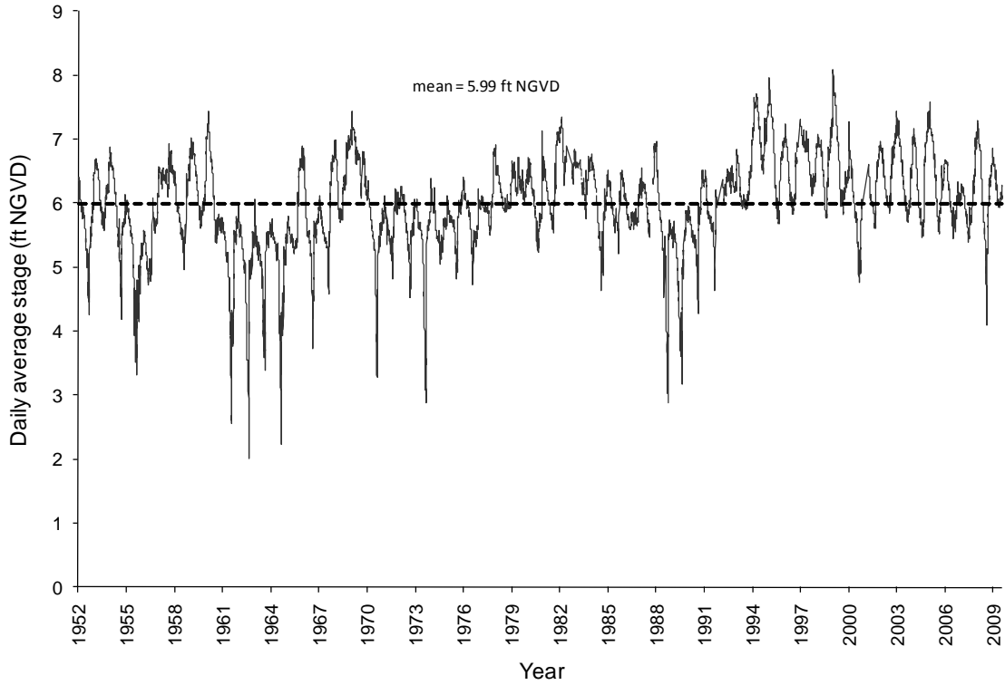
Figure 13. Daily average stage for Everglades National Park (ENP) (site P-33).
