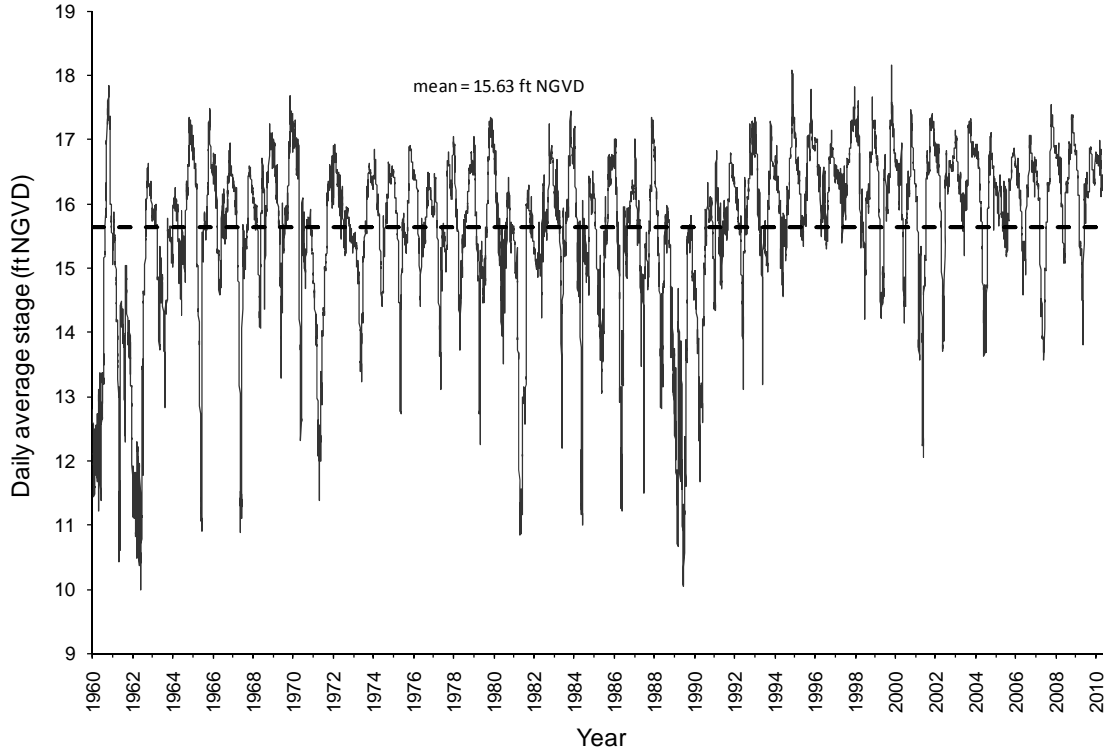
Figure 10. Daily average stage for Water Conservation Area 1 (sites 1-8C, 1-7, 1-8T, and 1-9).
