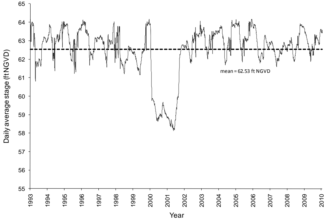
Figure 1. Daily average stage for Lake Alligator (site S60_H).
