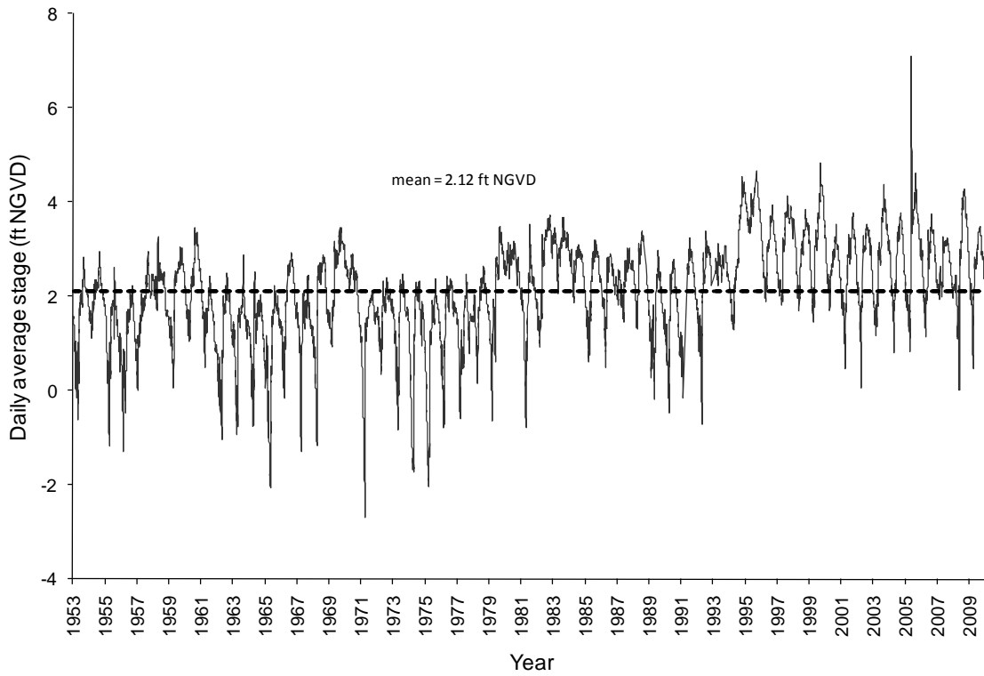
Figure 14. Daily average stage for the ENP (site P-34).
