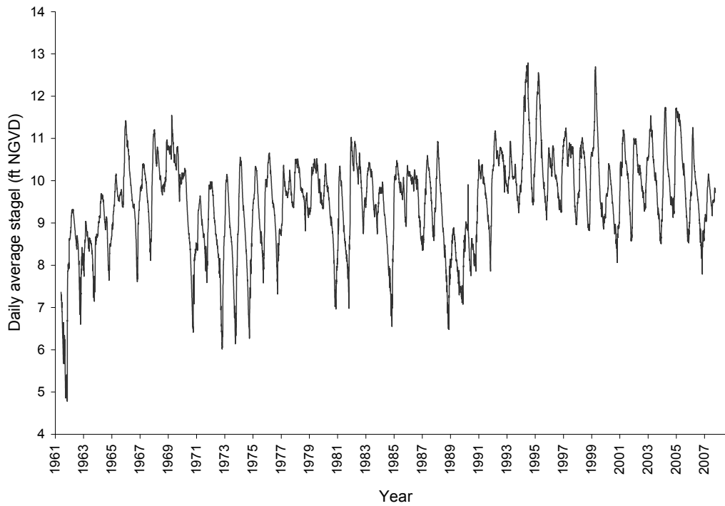
Figure 12. Daily average stage for Water Conservation Area 3A (CA3AVG).
