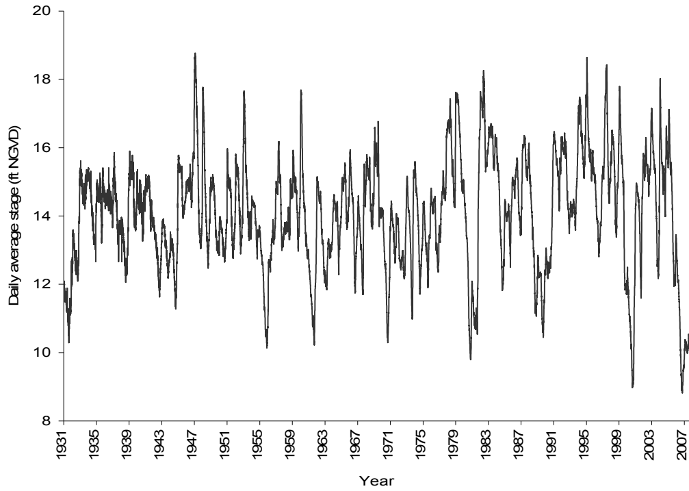
Figure 9. Daily average stage for Lake Okeechobee.
