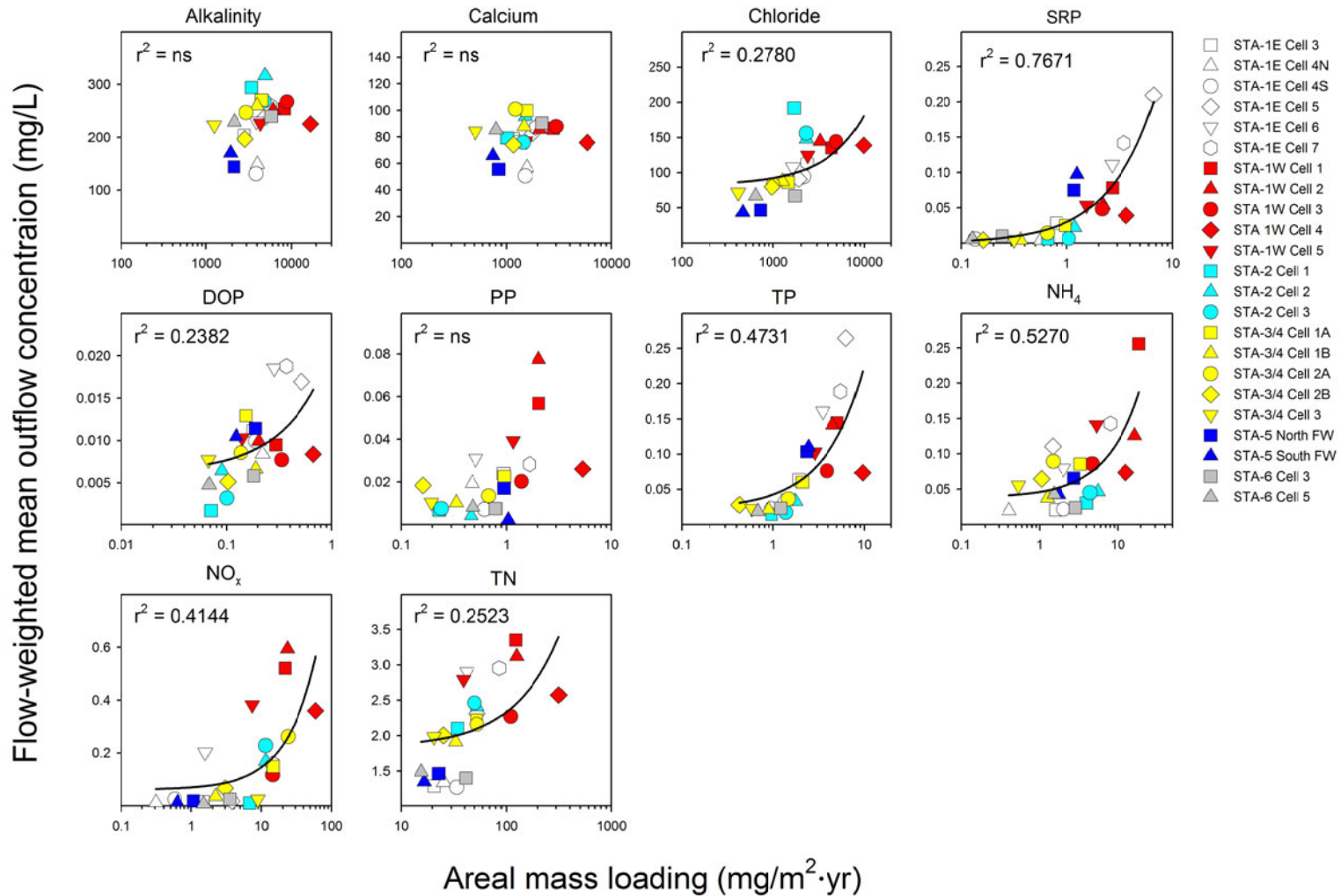
Figure 2. Period-of-record areal mass loading versus flow-weighted mean outflow concentration for constituents monitored in the STA flow-ways and treatment cells. Lines are linear fits through the data.
