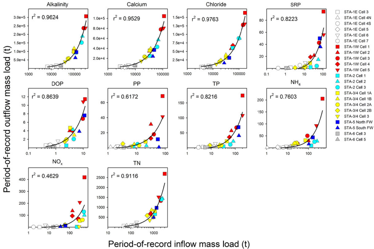
Figure 1. Period-of-record inflow versus outflow mass loads for constituents monitored in the (STA) flow-ways and treatment cells. Lines are linear fits through the data.
