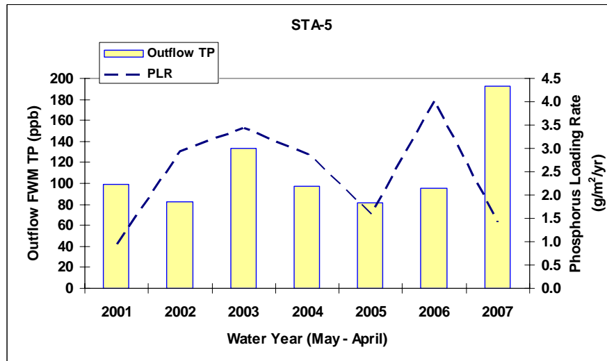
Figure 5. Continued. Flow, TP load, flow-weighted mean TP concentrations, and hydraulic and phosphorus loadings at Stormwater Treatment Area 5 (STA-5) during WY2001–WY2007. Sections of STA-5 were temporarily off-line during WY2004–WY2007. Refer to Chapter 5 of this volume for information about treatment cell status.
