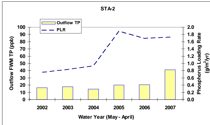
Figure 3. Continued. Flow, TP load, flow-weighted mean TP concentrations, and hydraulic and phosphorus loadings at Stormwater Treatment Area 2 (STA-2) during WY2002–WY2007. All treatment cells were operational during WY2007.
