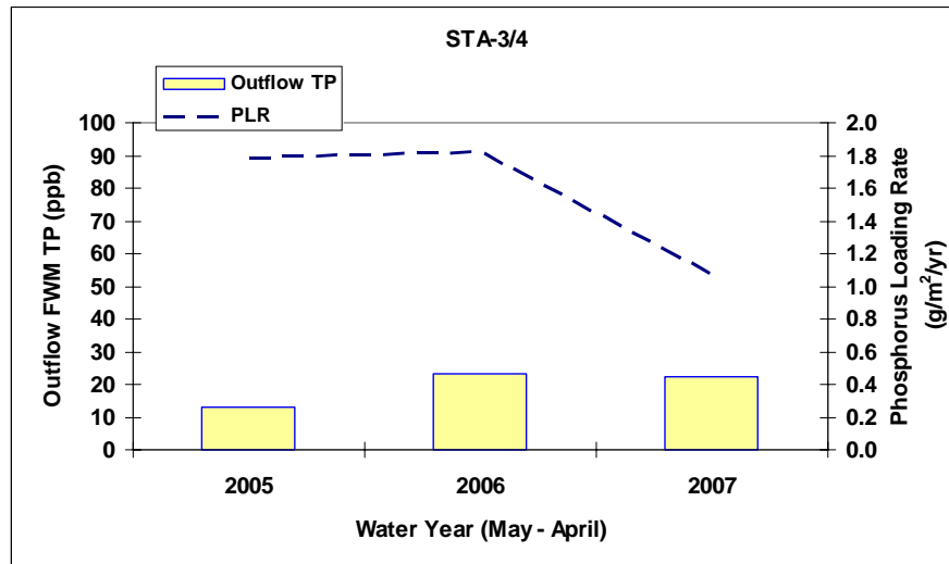
Figure 4. Continued. Flow, TP load, flow-weighted mean TP concentrations, and hydraulic and phosphorus loadings at Stormwater Treatment Area 3/4 (STA-3/4) during WY2005–WY2007. All treatment cells were operational during WY2007. Refer to Chapter 5 in this volume for information about treatment cell status in prior water years.
