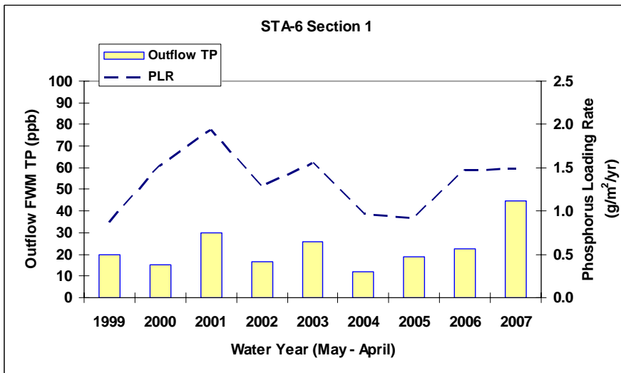
Figure 6. Continued. Flow, TP load, flow-weighted mean TP concentrations, and hydraulic and phosphorus loadings at Stormwater Treatment Area 6 (STA-6) during WY1999–WY2007. Sections of STA-6 were temporarily off-line during WY2007. Refer to Chapter 5 of this volume for information about treatment cell status.
