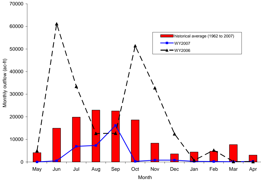
Figure 7. Monthly outflow from C-25 (site S-50).
