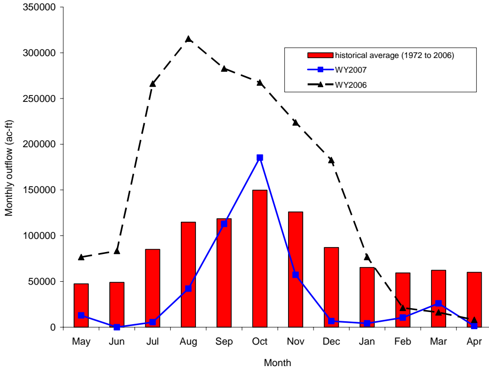
Figure 15. Monthly outflow from WCA-3.
