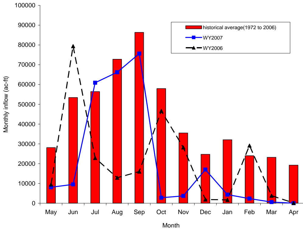
Figure 10. Monthly inflow into Water Conservation Area 1 (WCA-1).
