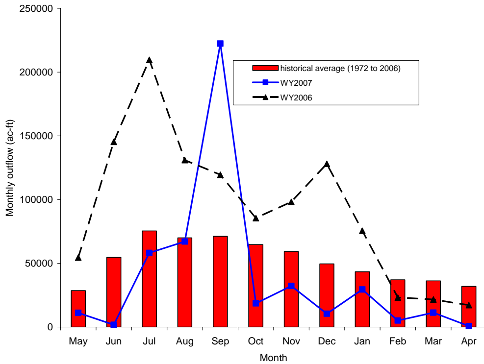
Figure 12. Monthly inflow to WCA-2.
