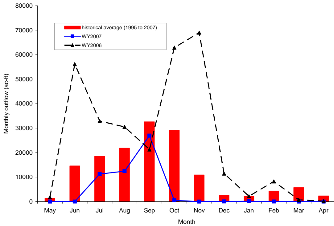
Figure 5. Monthly outflow from C-23 (site S-48).
