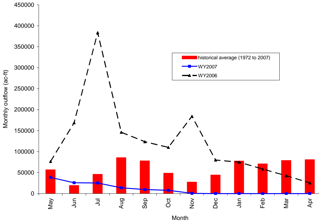
Figure 1. Monthly outflow from Lake Kissimmee.
