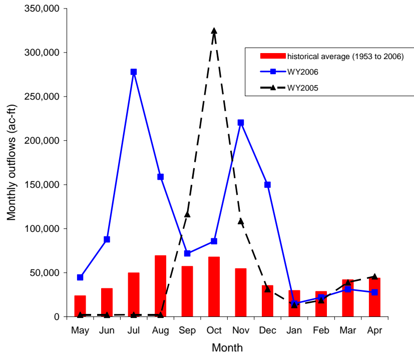
Figure 8. Monthly outflow from C-44 (site S-80).
