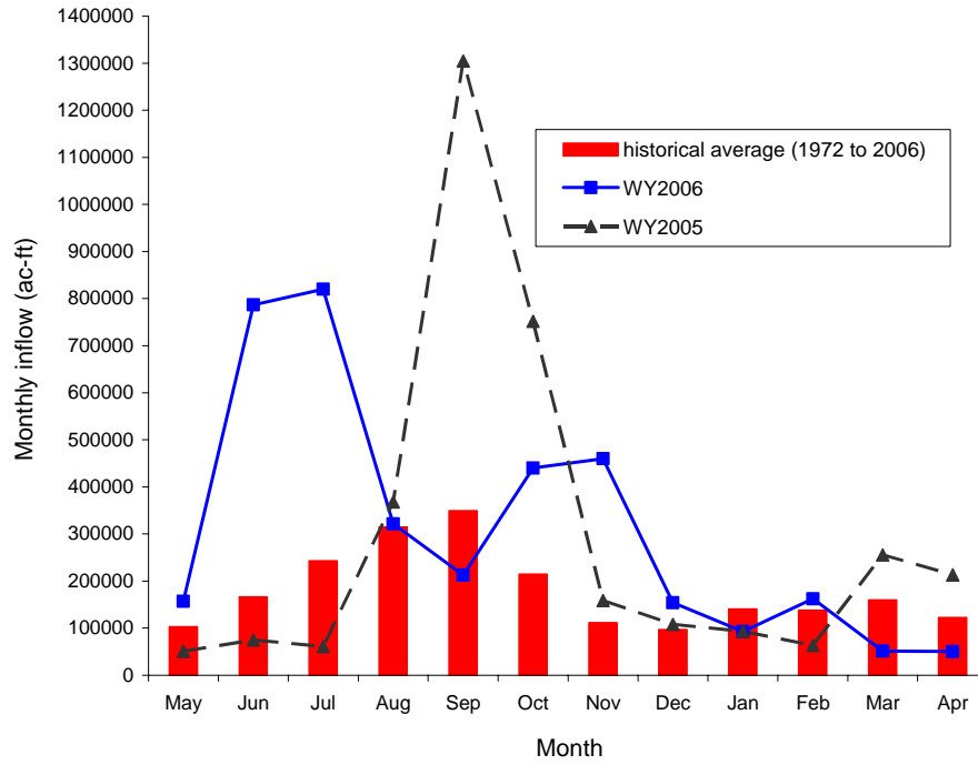
Figure 3. Monthly inflow to Lake Okeechobee.
