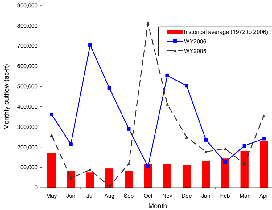
Figure 4. Monthly outflow from Lake Okeechobee.
