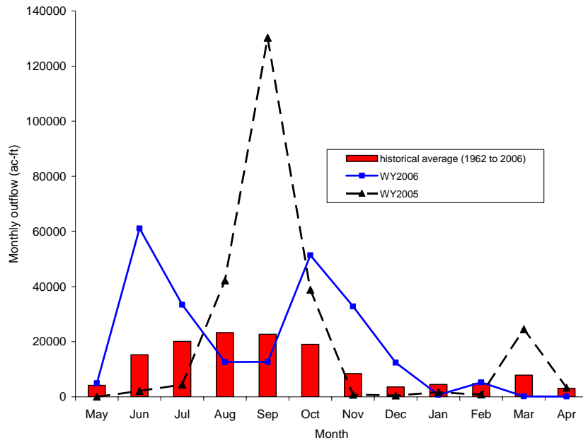
Figure 7. Monthly outflow from C-25 (site S-50).
