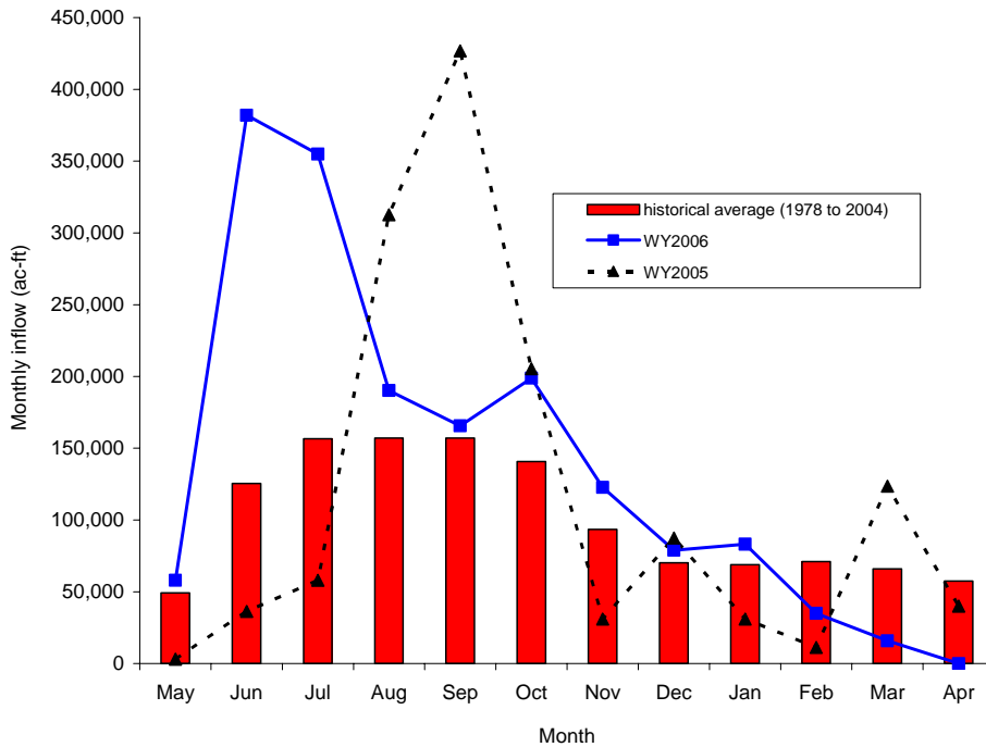
Figure 14. Monthly inflow to WCA-3A.
