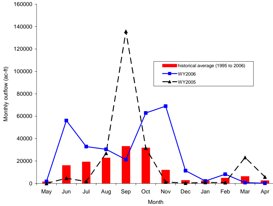
Figure 5. Monthly outflow from C-23 (site S-48).
