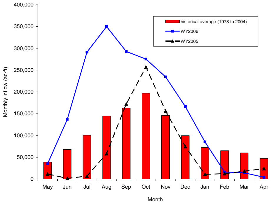
Figure 16. Monthly inflow to Everglades National Park.
