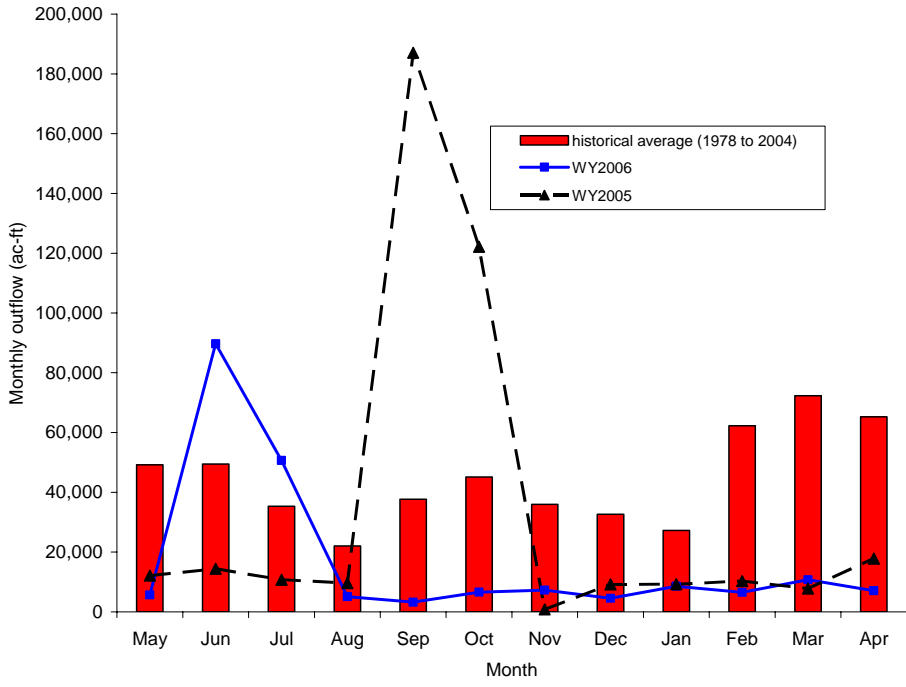
Figure 11. Monthly outflow from WCA-1.
