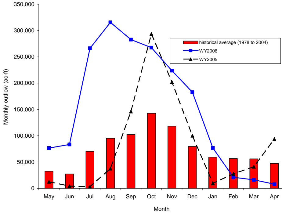
Figure 15. Monthly outflow from WCA-3A.
