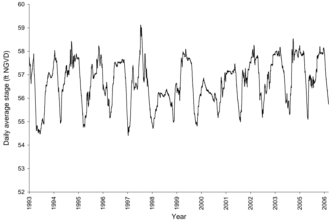
Figure 5. Daily average stage for East Lake Tohopekaliga.
