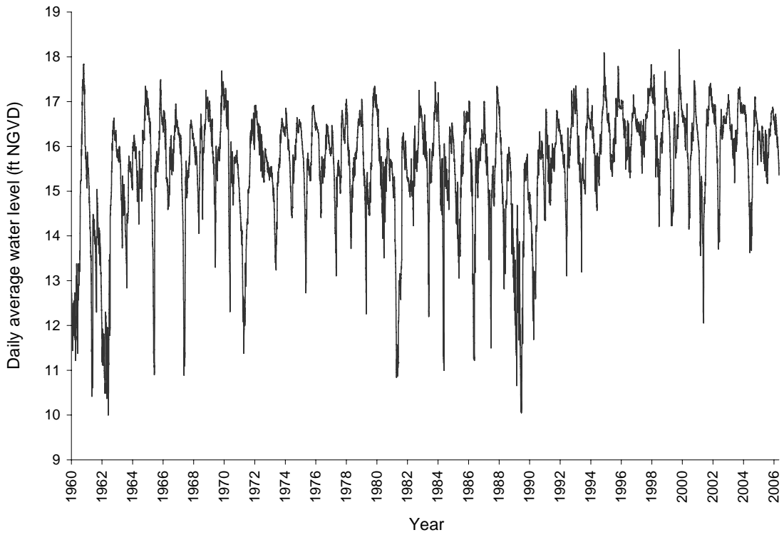
Figure 10. Daily average stage for Water Conservation Area 1.
