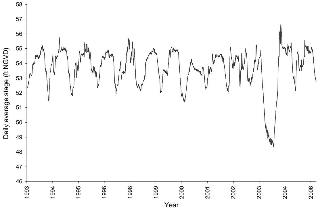
Figure 6. Daily average stage for Lake Tohopekaliga.
