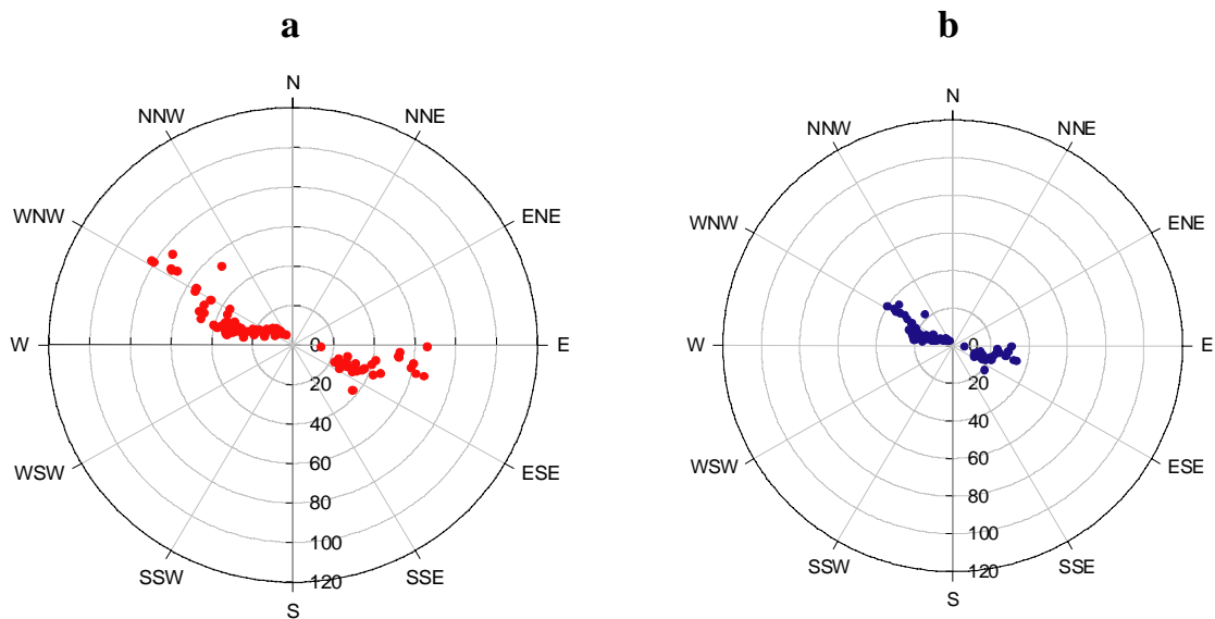
Figure 29. (a) Maximum wind gust speed (mph), (b) average wind speed (mph) and wind direction at BIG CY SIR weather station during Hurricane Wilma at 15-minute interval (October 24, 2005).
