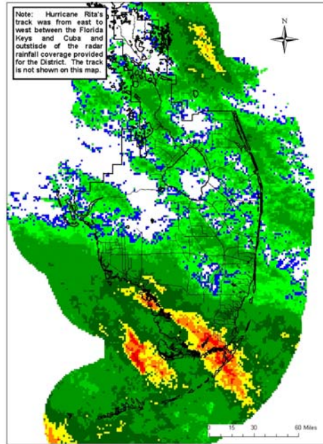
Figure 2c. Radar rainfall from Hurricane Rita as it passed through the Florida Straits (September 19-21, 2005).
