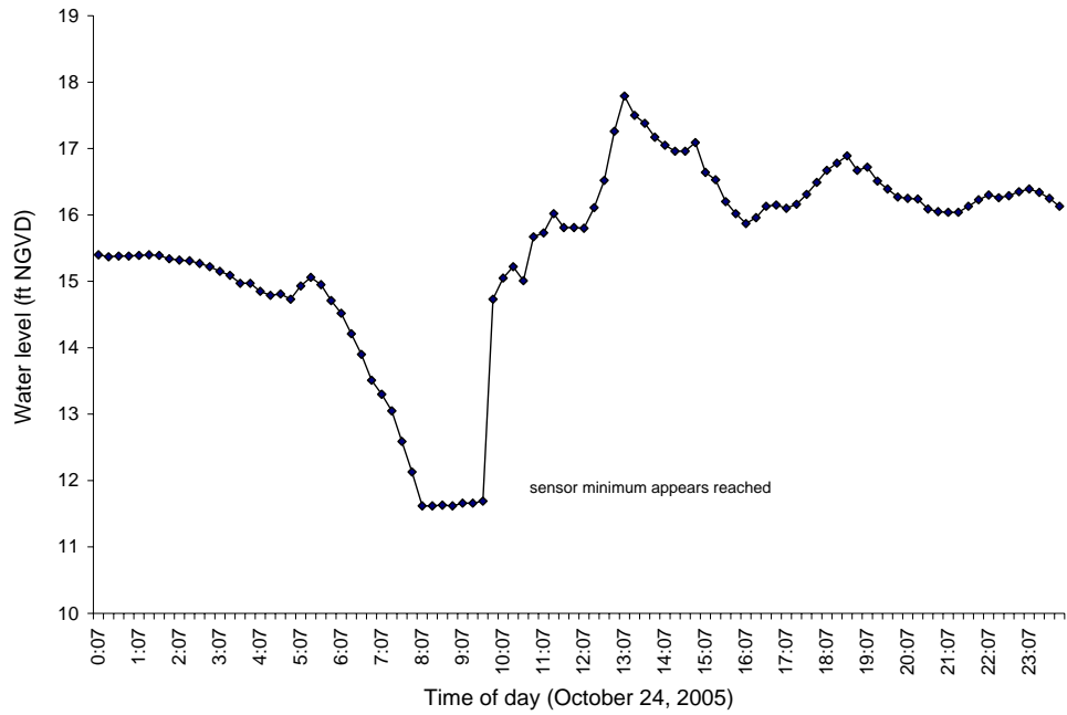
Figure 50. Lake Okeechobee water level changes at the S-135 structure during Hurricane Wilma.
