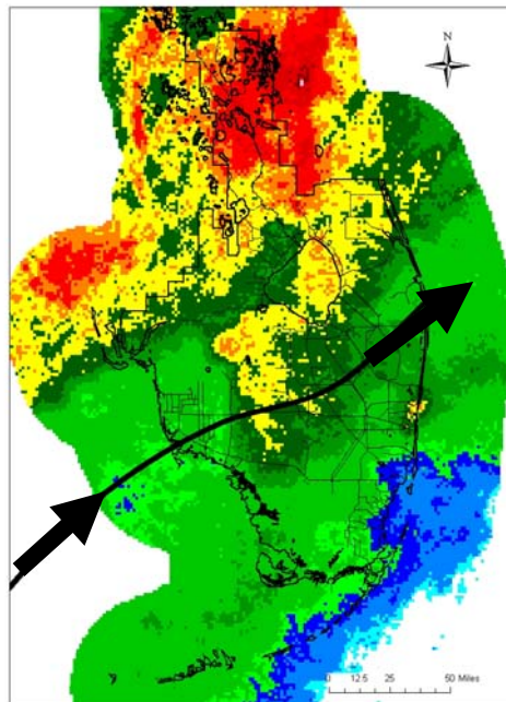
Figure 2d. Hurricane Wilma path and radar rainfall (October 22-25, 2005).
