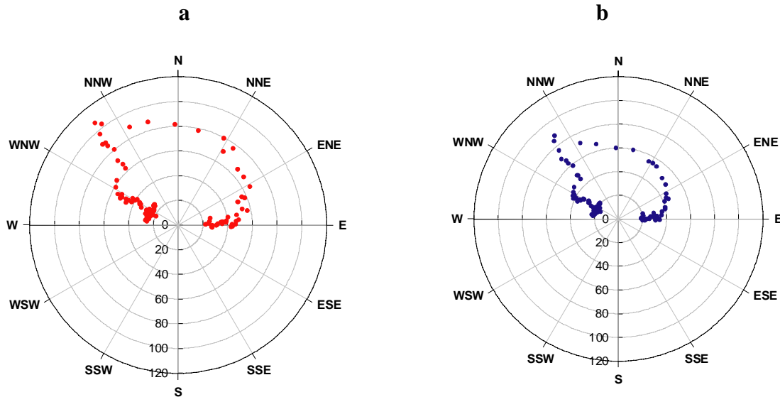
Figure 42. (a) Maximum wind gust speed (mph), (b) average wind speed (mph) and wind direction at L001 weather station during Hurricane Wilma at 15-minute interval (October 24, 2005).
