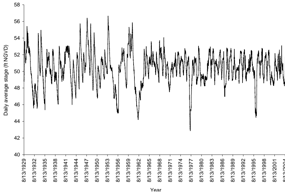
Figure 7. Daily average stage for Lake Kissimmee.
