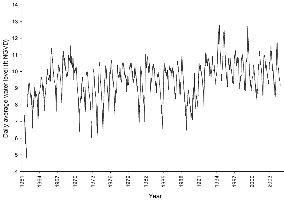
Figure 12. Daily average stage for Water Conservation Area 3.
