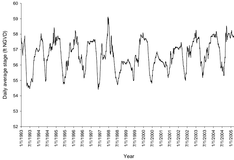
Figure 5. Daily average stage for Lake East Tohopekaliga.
