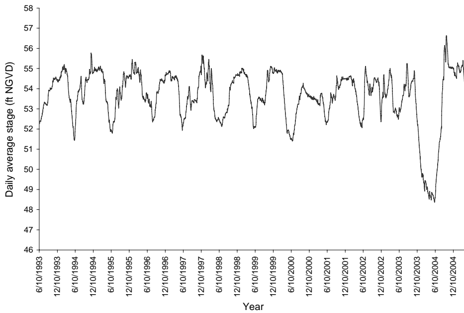
Figure 6. Daily average stage for Lake Tohopekaliga.
