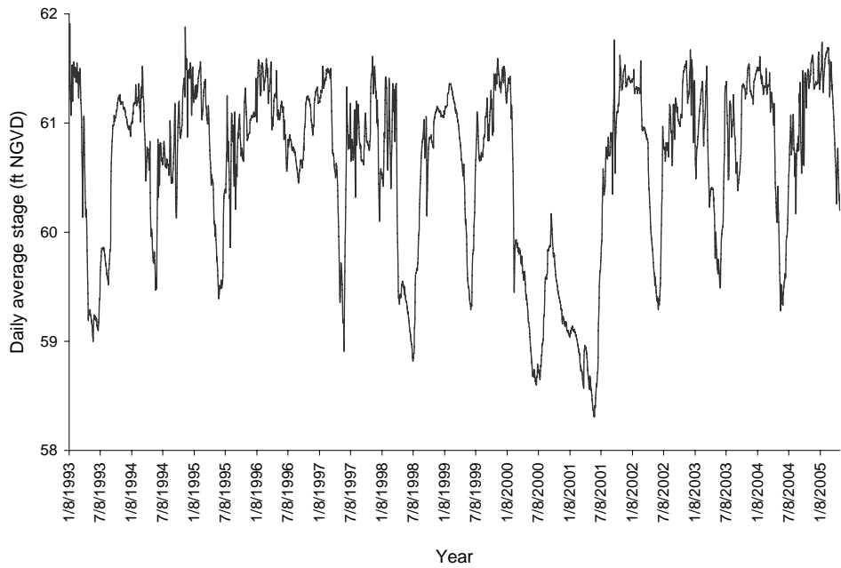
Figure 4. Daily average stage for Lake Gentry.
