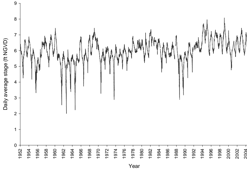
Figure 13. Daily average stage for ENP at site P33.
