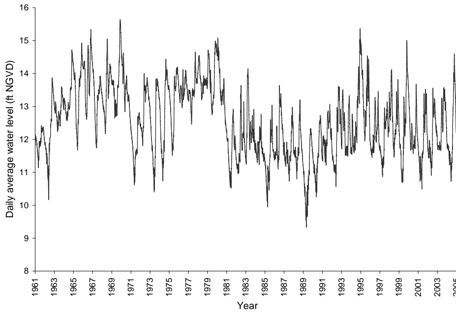
Figure 11. Daily average stage for Water Conservation Area 2.
