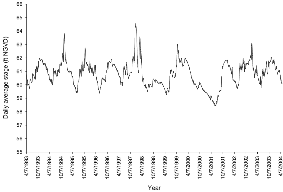
Figure 2. Daily average stage for Lake Myrtle.
