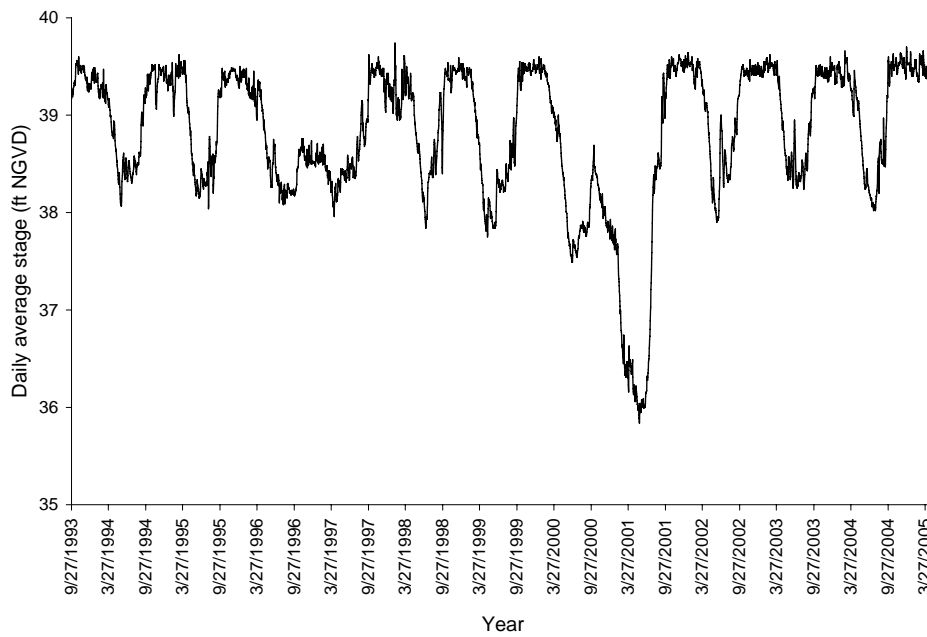
Figure 8. Daily average stage for Lake Istokpoga.
