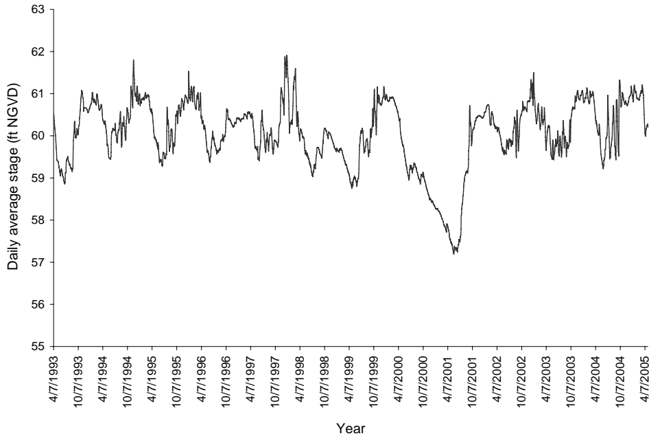
Figure 3. Daily average stage for Lake Mary Jane.
