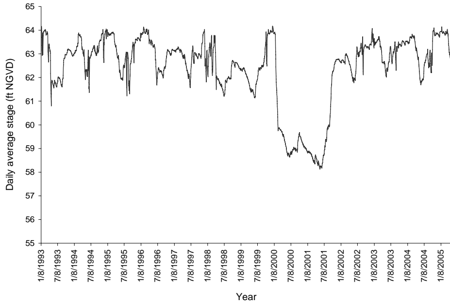
Figure 1. Daily average stage for Lake Alligator.
