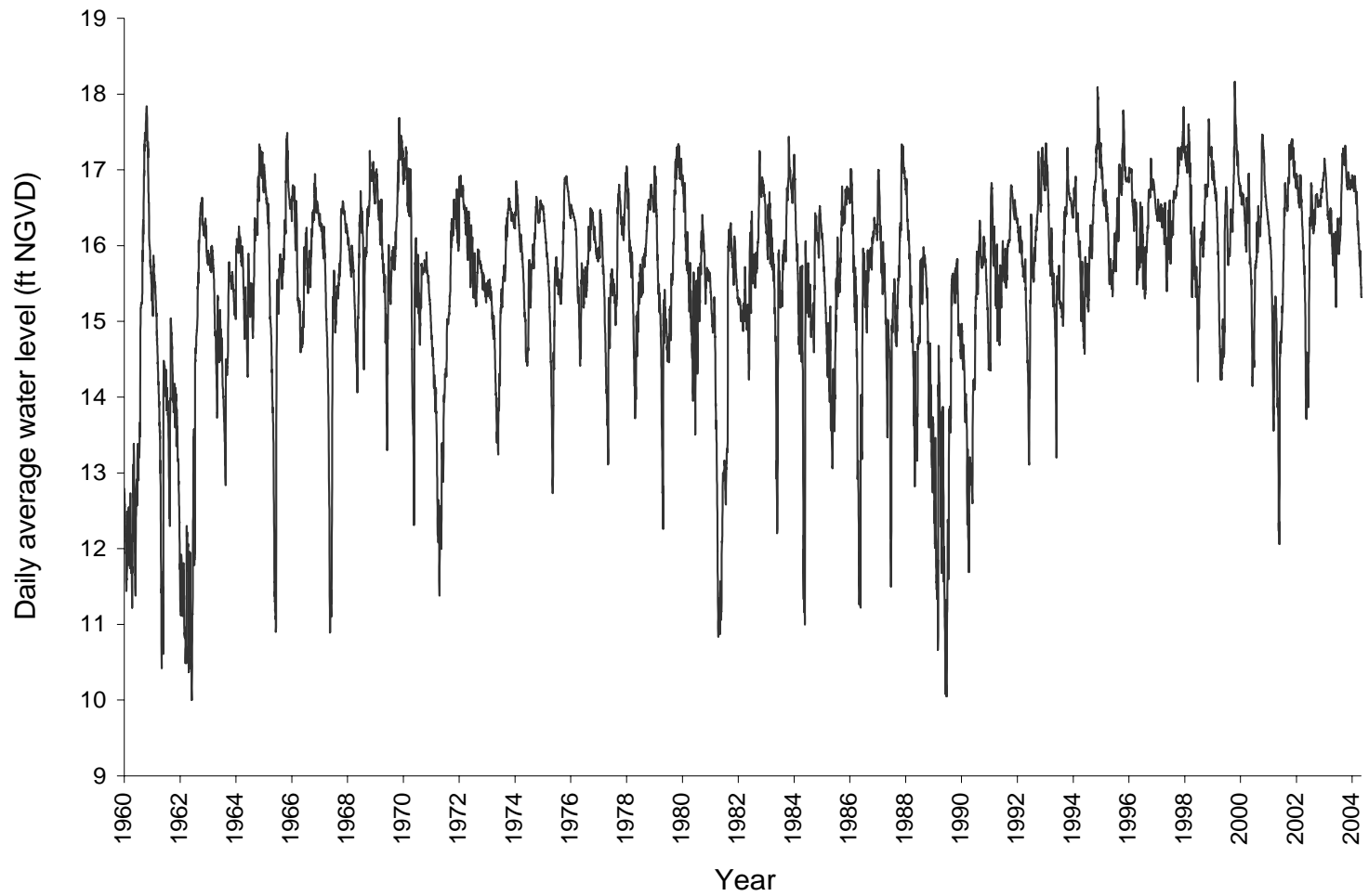
Figure 10. Daily average stage for Water Conservation Area 1.
