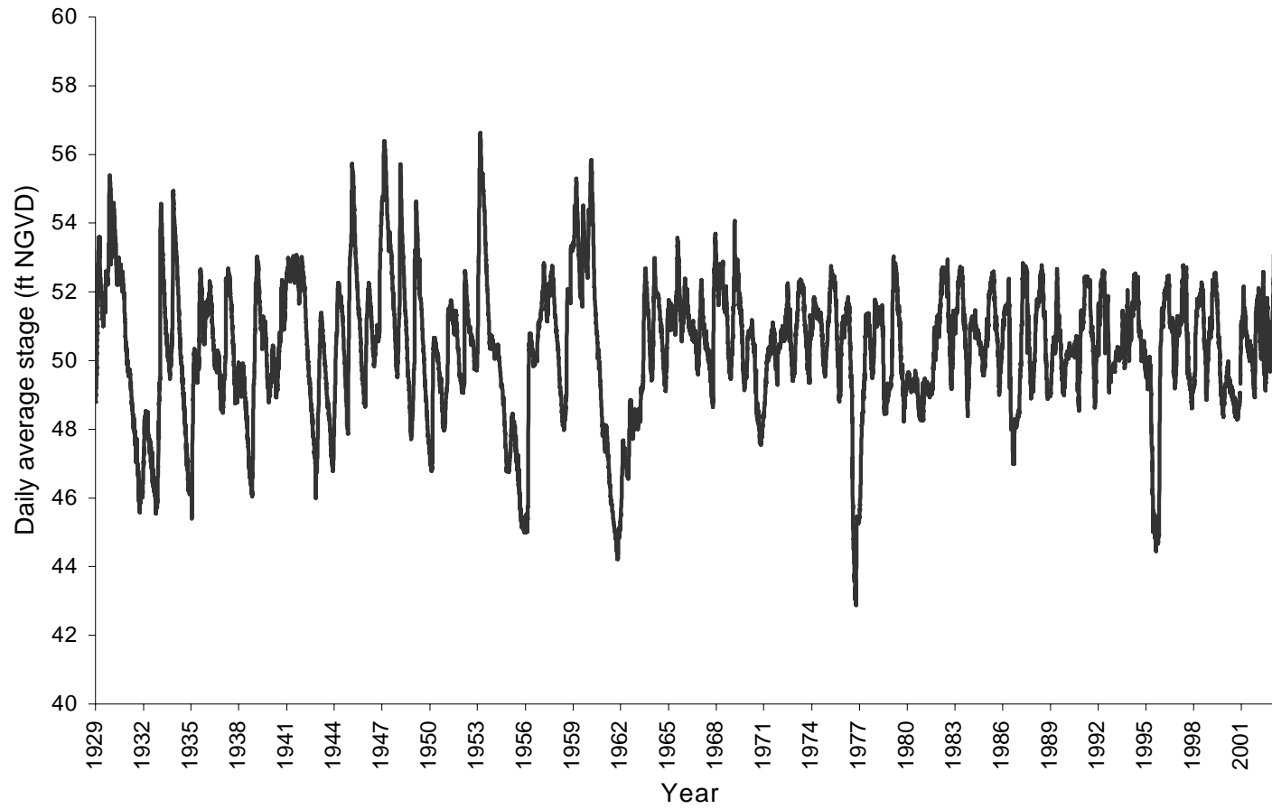
Figure 7. Daily average stage for Lake Kissimmee.
