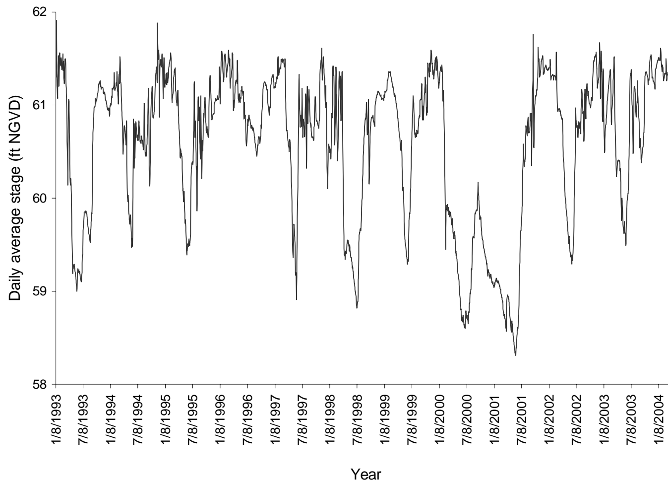
Figure 4. Daily average stage for Lake Gentry.
