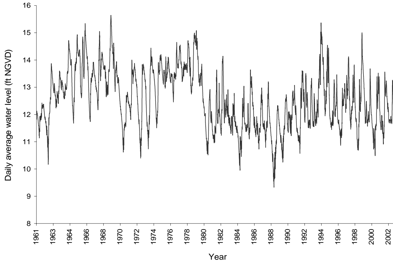
Figure 11. Daily average stage for Water Conservation Area 2.
