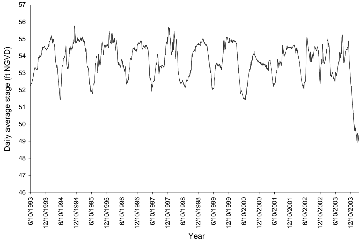
Figure 6. Daily average stage for Lake Tohopekaliga.
