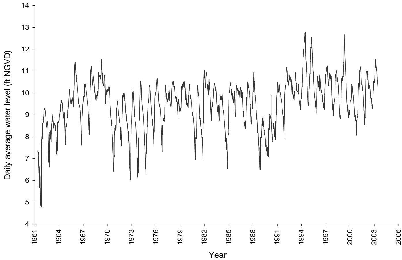
Figure 12. Daily average stage for Water Conservation Area 3.
