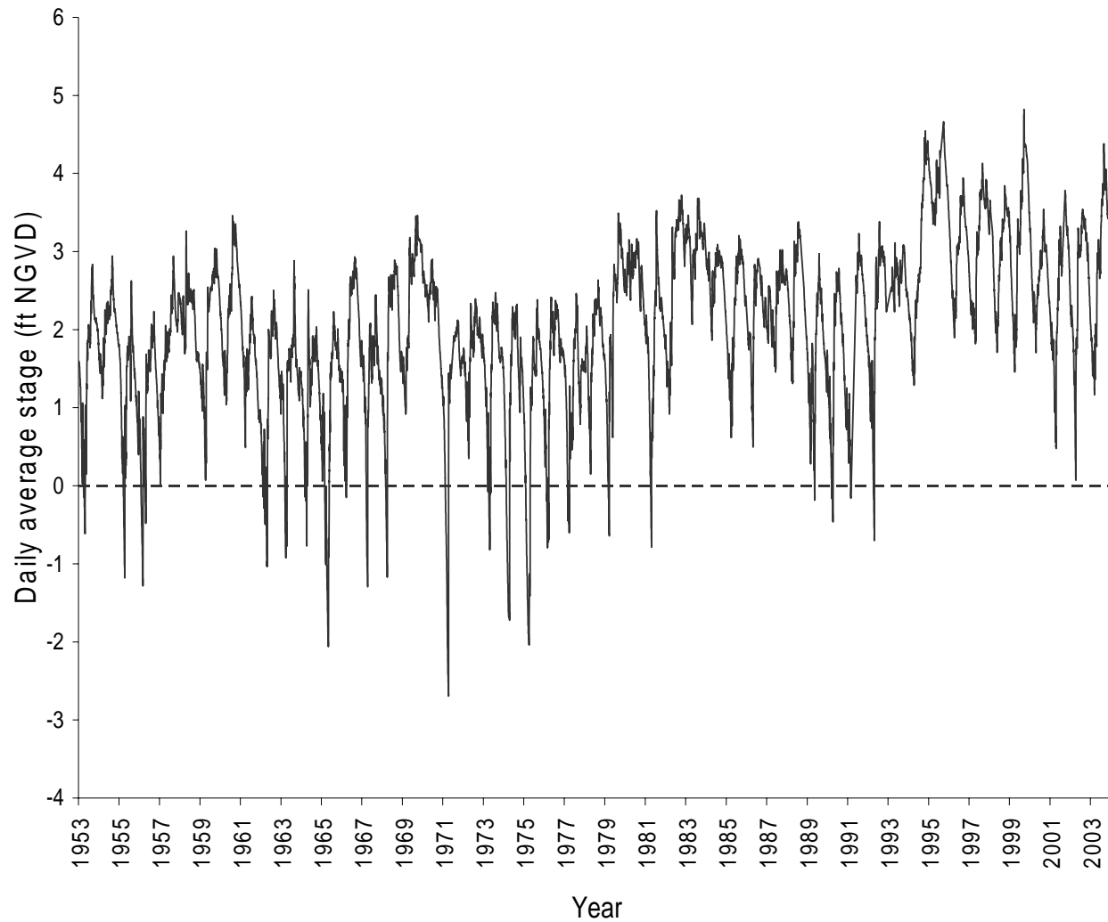
Figure 14. Daily average stage for Everglades National Park at site P-34.
