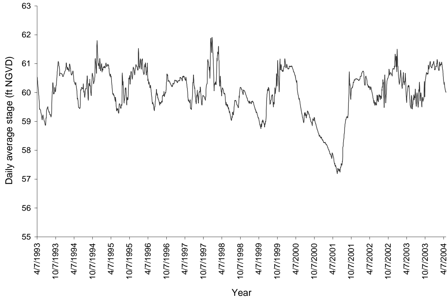
Figure 3. Daily average stage for Lake Mary Jane.
