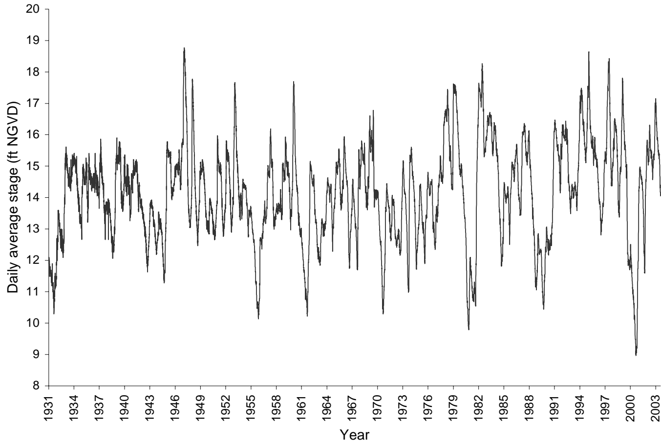
Figure 9. Daily average stage for Lake Okeechobee.
