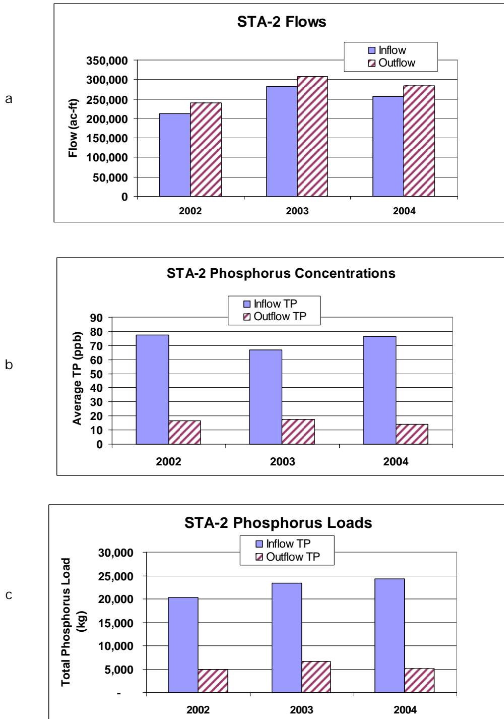
Figure 2. Time series plots showing flow (a), and TP load (b) and concentration (c) for STA-2 (2002–2004).
